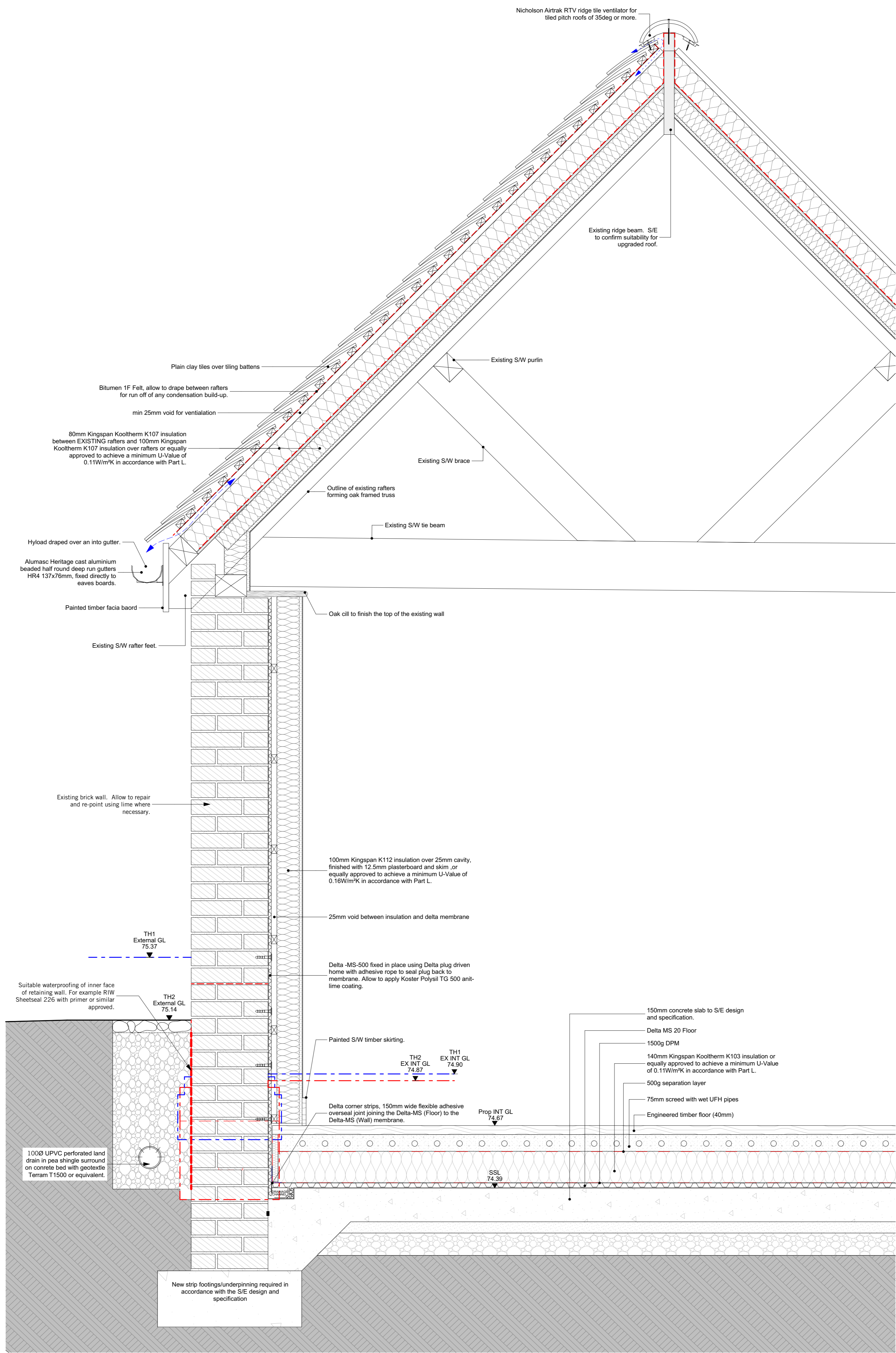
D04 Games Room Floor Wall and Roof 1:10
