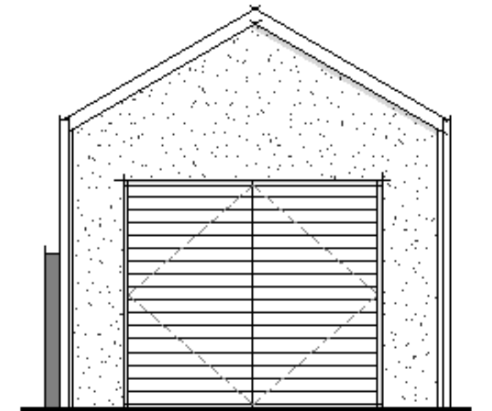
Rear Elevation at 1:50
