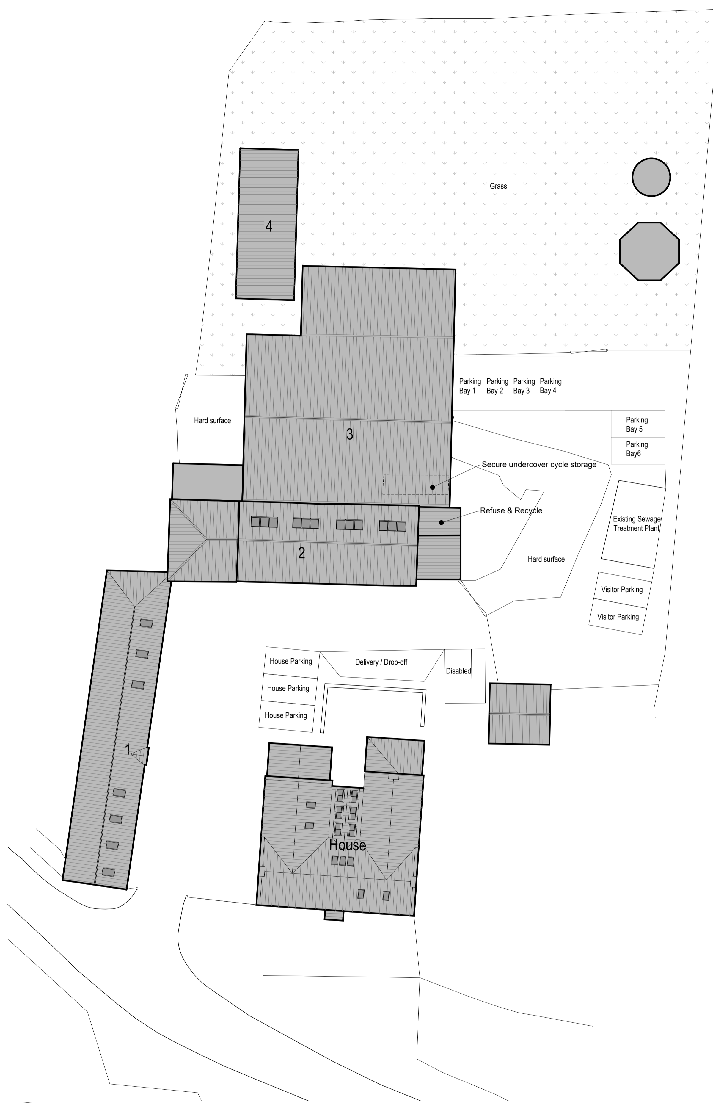
B Proposed Block Plan/Roof Plan 1:200
