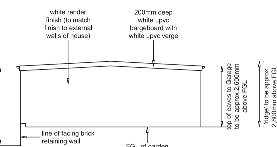
GARAGE:- West Elevation
