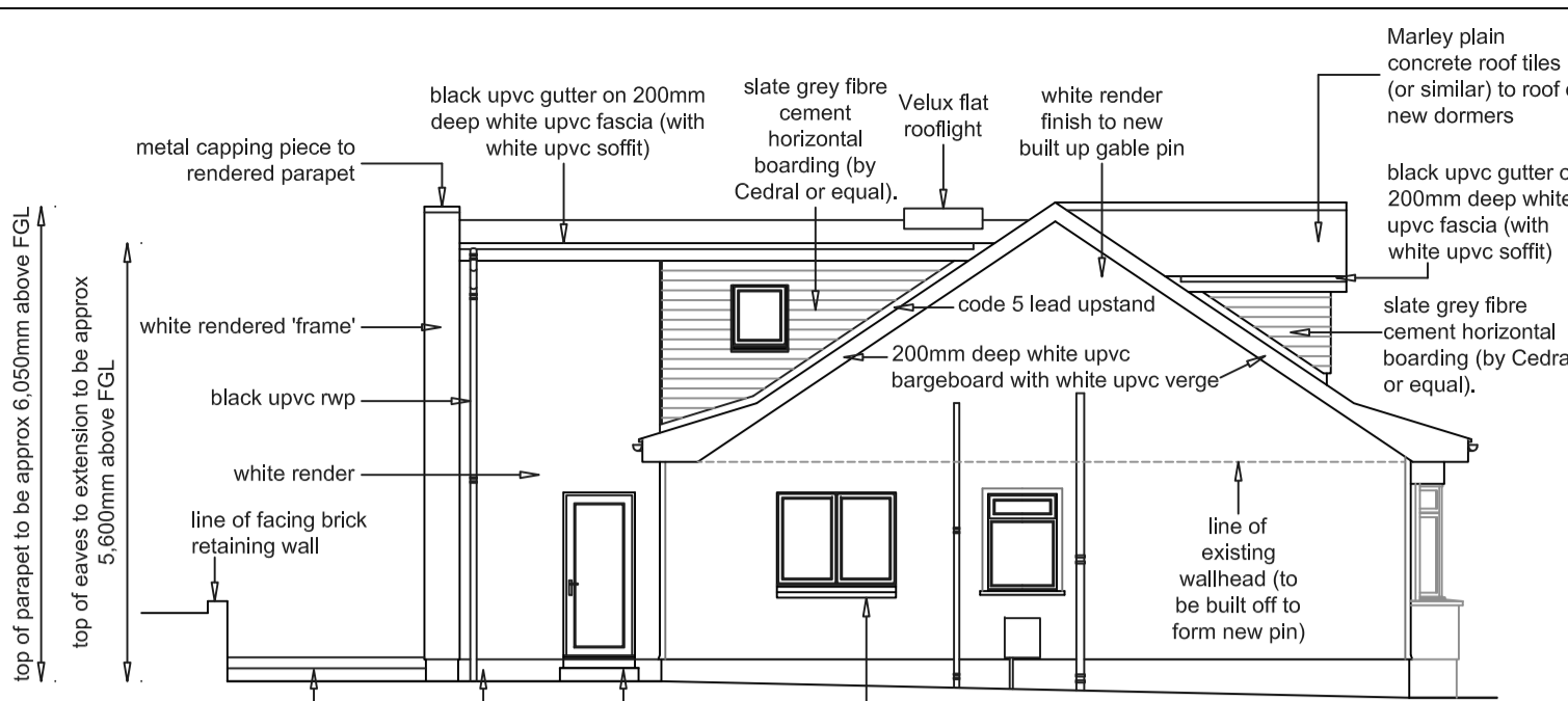
HOUSE:- East Elevation
