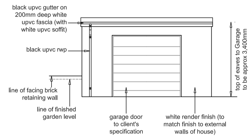
GARAGE:- Front Elevation
