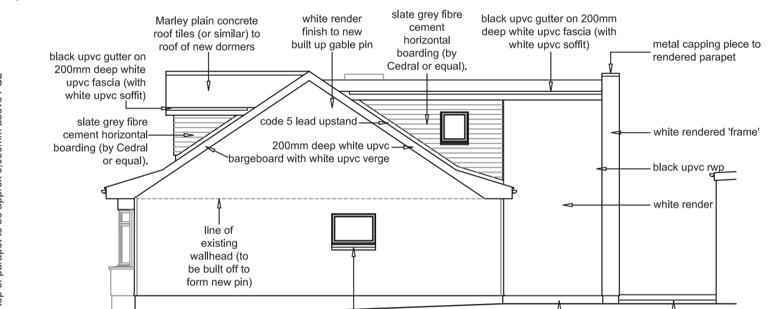
HOUSE:- West Elevation
