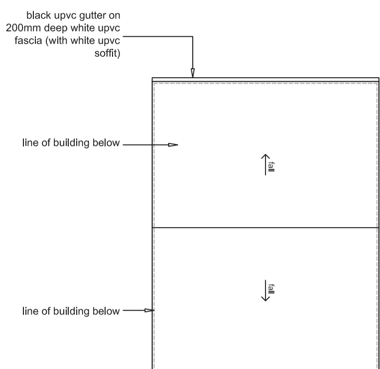
GARAGE:- Roof Plan
