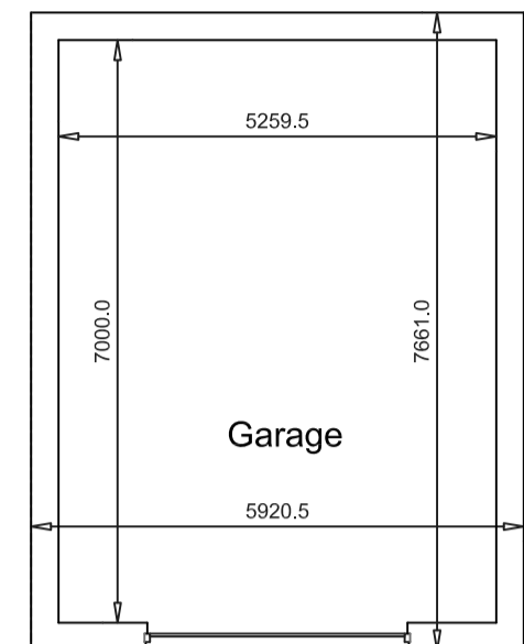
GARAGE:- Plan
