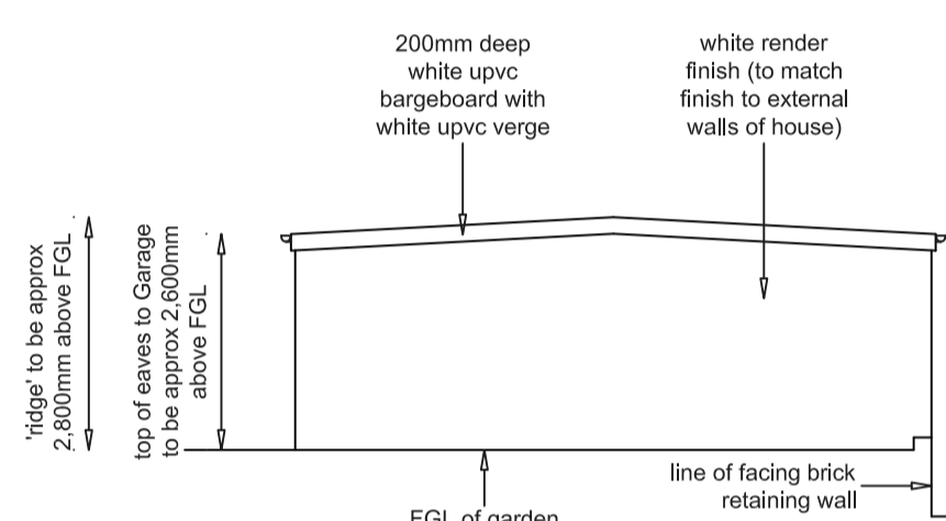
GARAGE:- East Elevation
