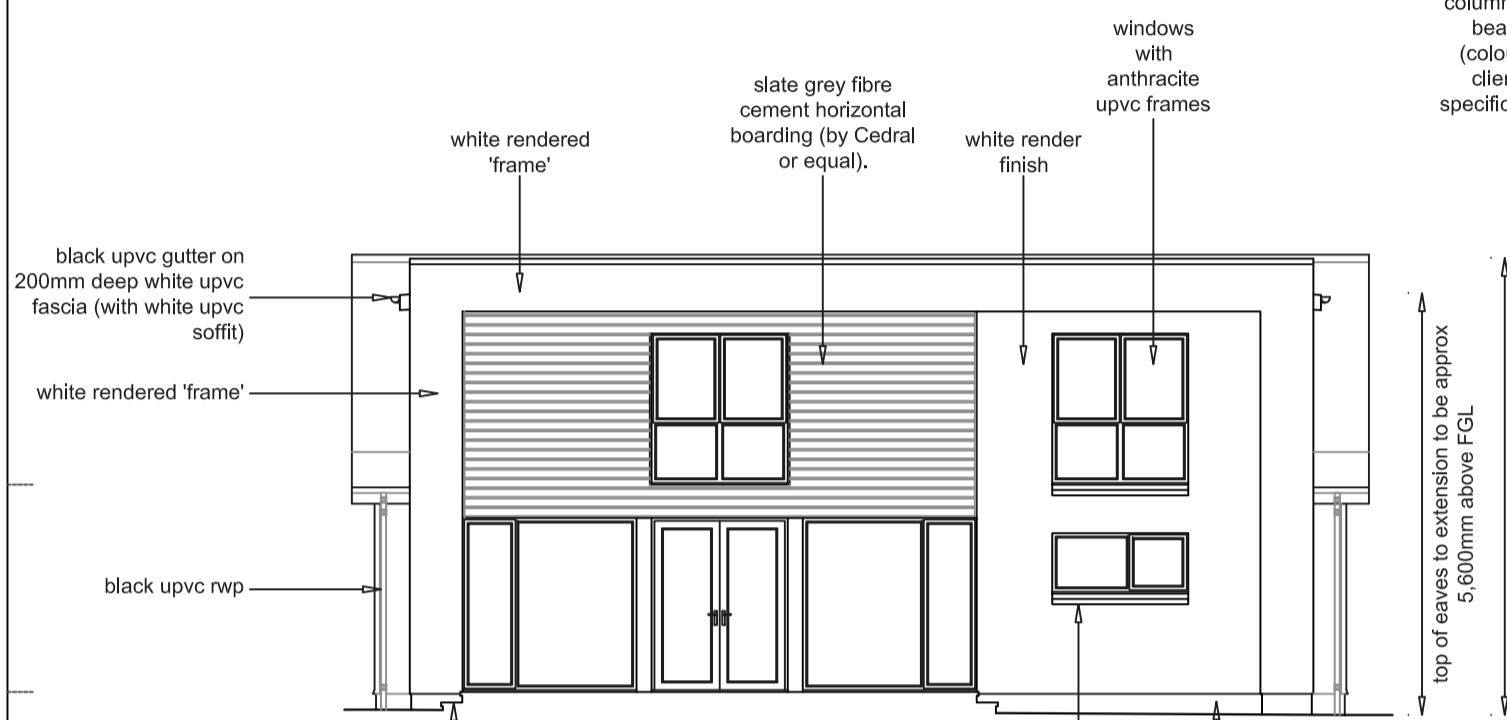
HOUSE:- Rear (South) Elevation
