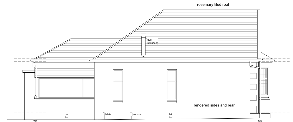
Side Elevation 1 : 100
