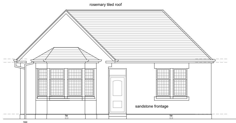
Front Elevation 1 : 100
