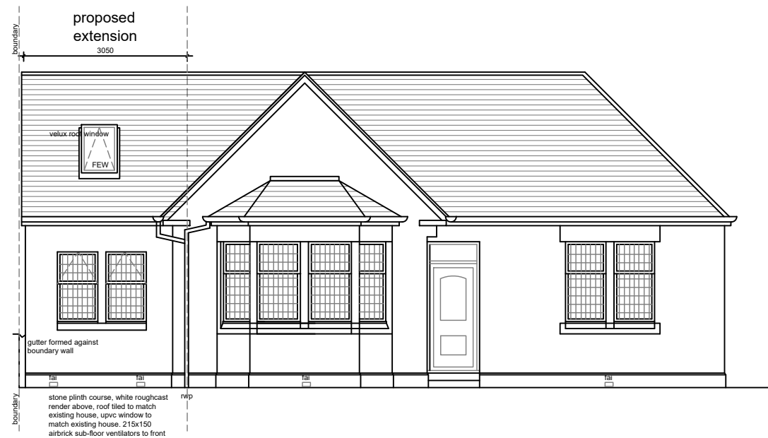
Front Elevation 1 : 100
