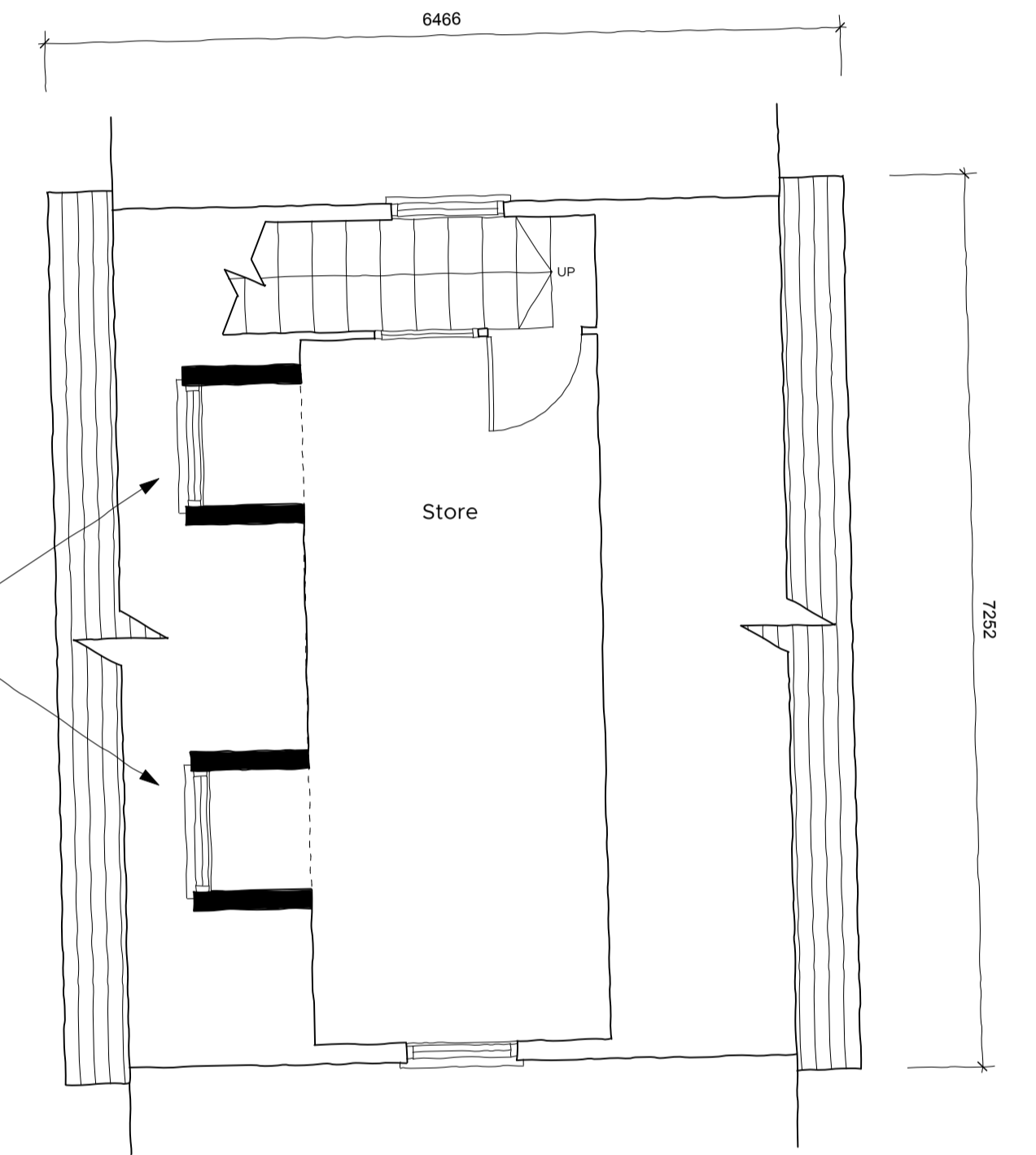
PROPOSED FIRST FLOOR PLAN - GARDEN ROOM
