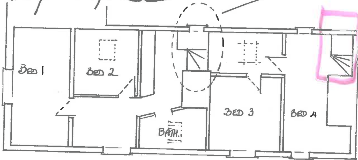
FIRST FLOOR PLAN 1:100 - REVISED ROOM LAYOUT - POSITION OF PROPOSED SKYLIGHTS
