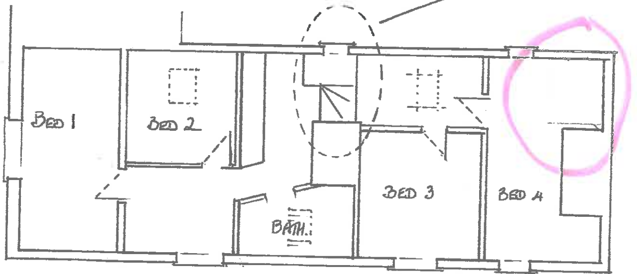
FIRST FLOOR PLAN 1:100 - REVISED ROOM LAYOUT - POSITION OF PROPOSED ROOFLIGHTS
