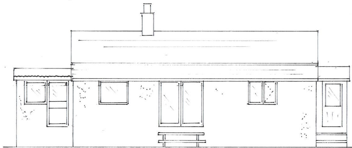
BACK VIEW
