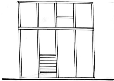
SOUTH ELEVATION 1:50
