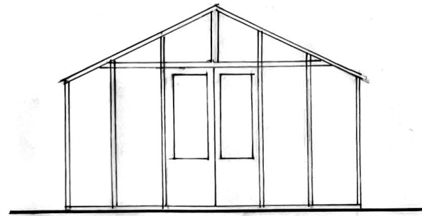
EAST ELEVATION 1:50
