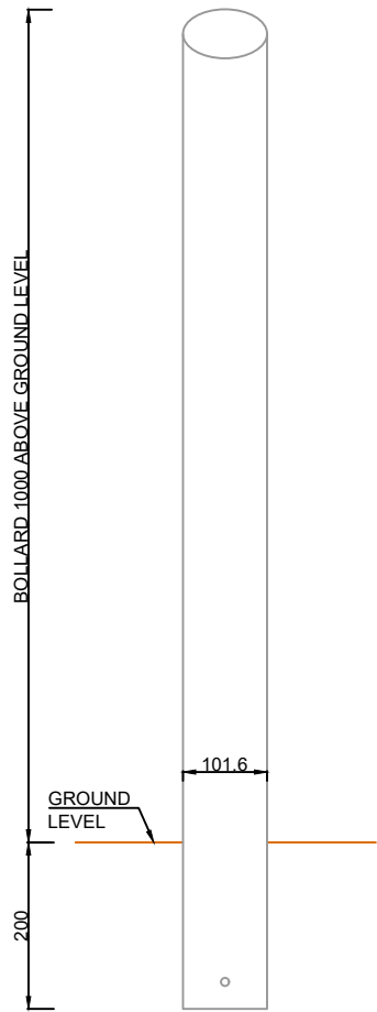
FRONT VIEW 1:10
