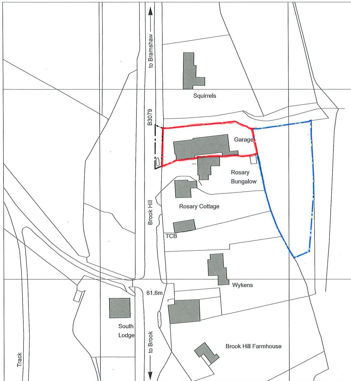
location plan 1:1250
