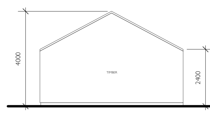
PROPOSED GARDEN MAINTENANCE STORE / WORKSHOP
