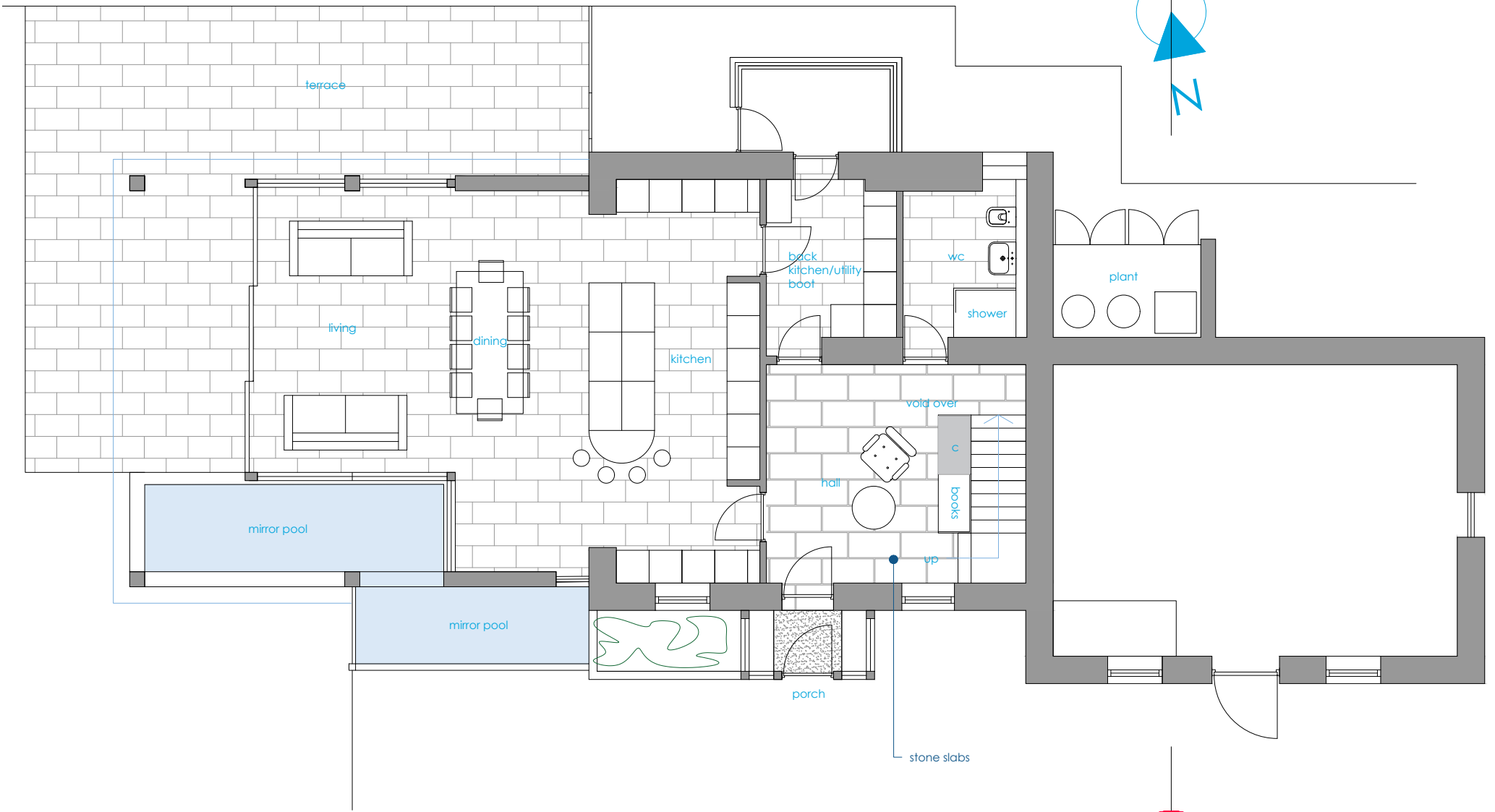
1:100 Ground floor plan
