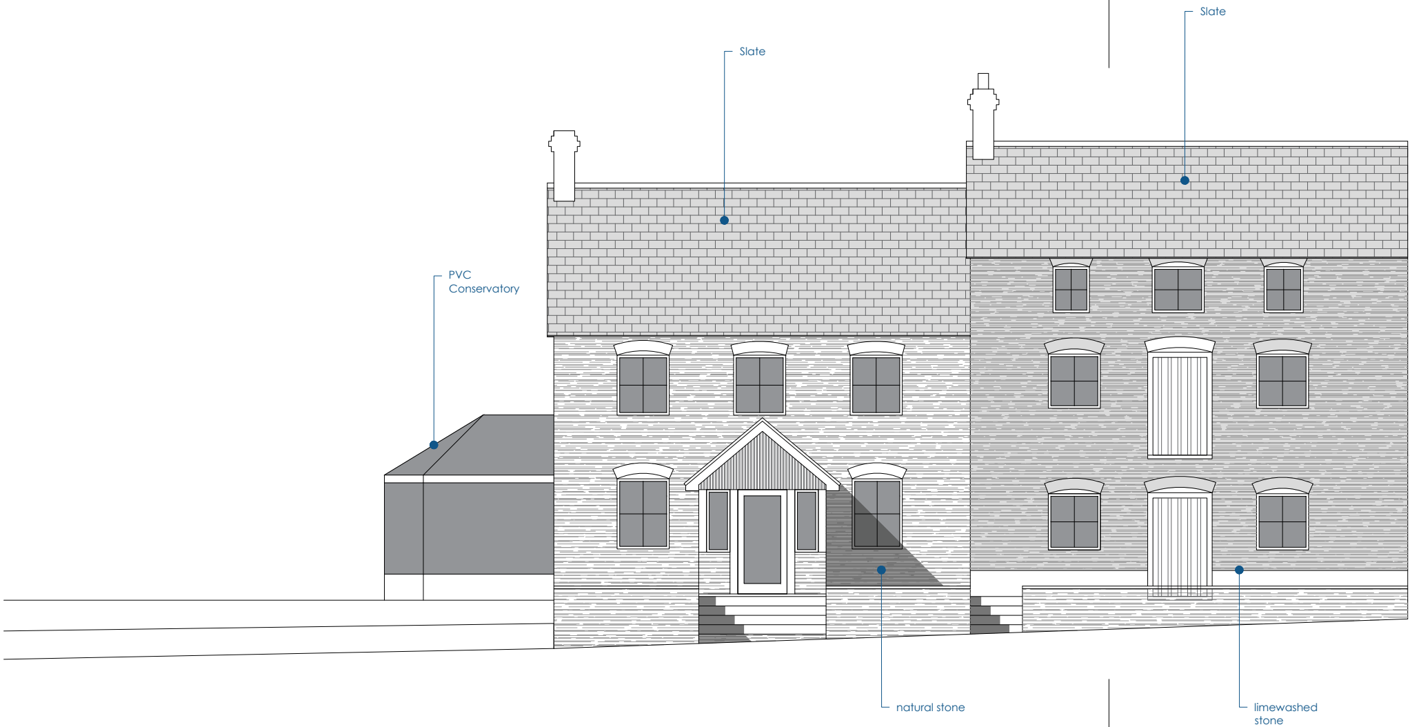
1:100 South Elevation
