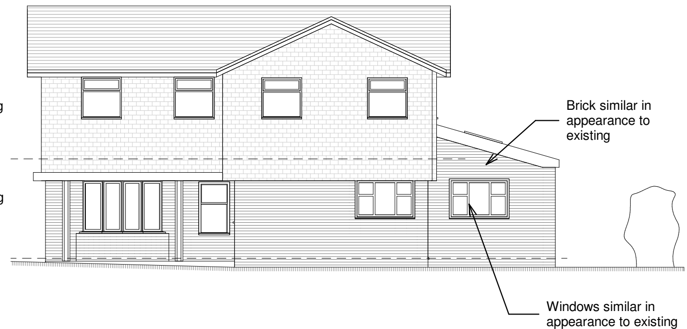
FRONT ELEVATION (SOUTH)
