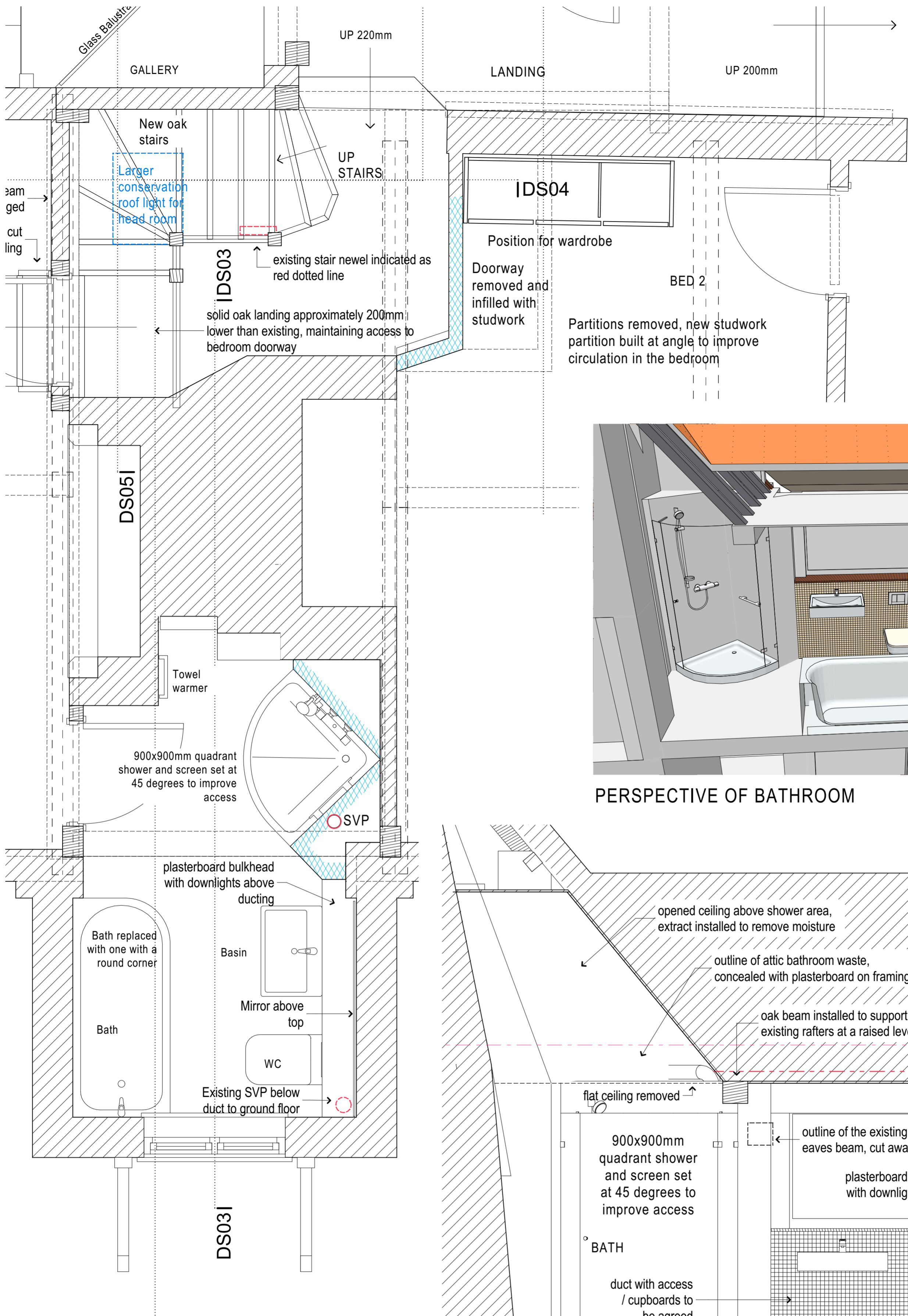
PLANS OF BATHROOM / BEDROOM 2
