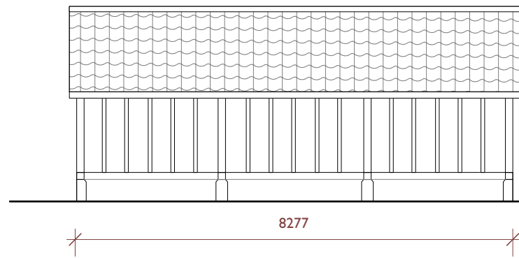
Rear Elevation
