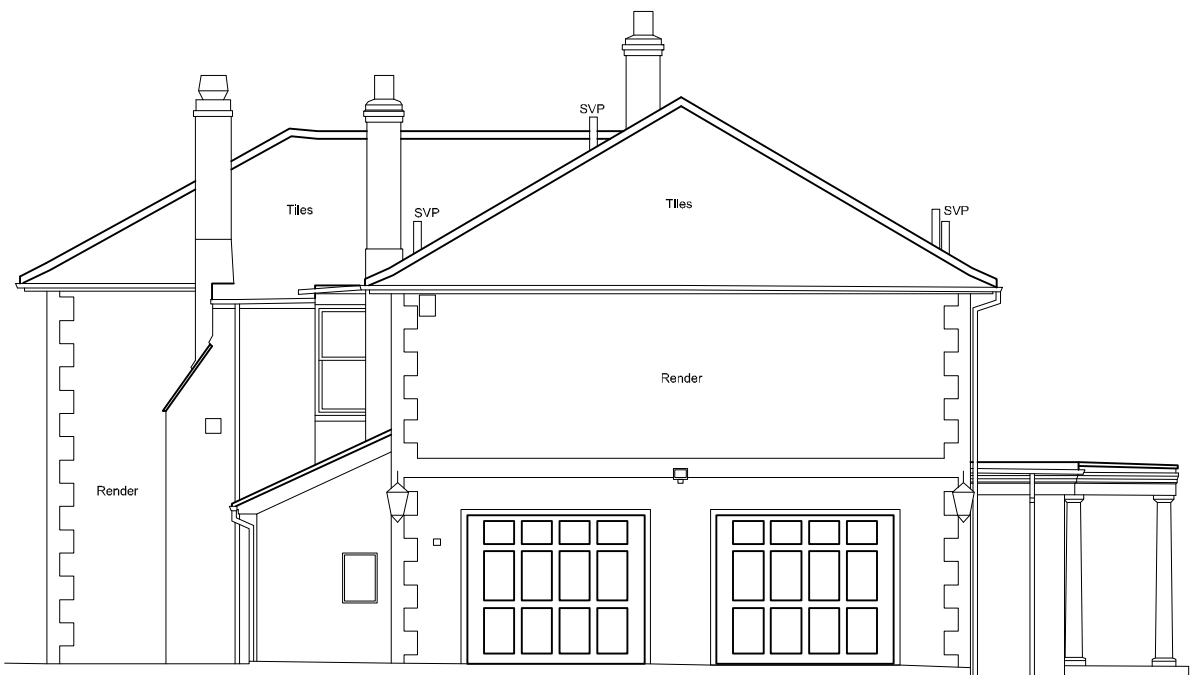
NORTH ELEVATION
