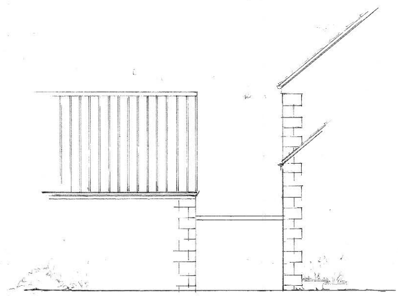
SOUTH ELEVATION
