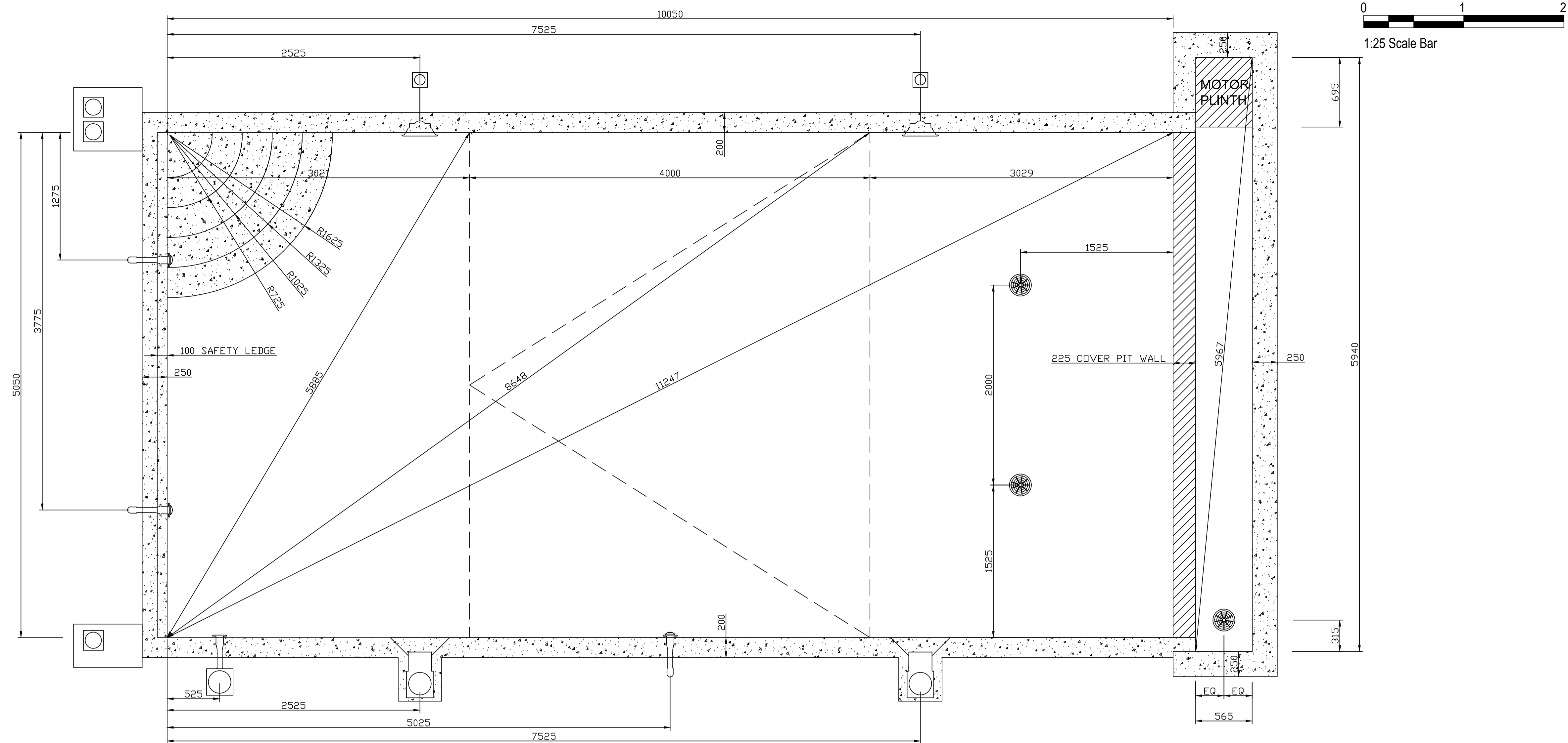
PLAN - POOL STRUCTURE
