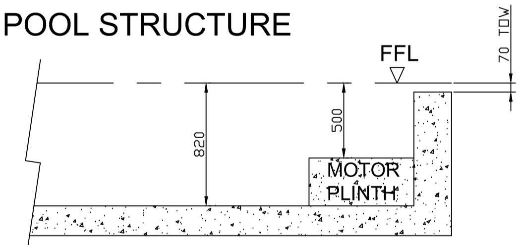
SECTION AA - COVER PIT
