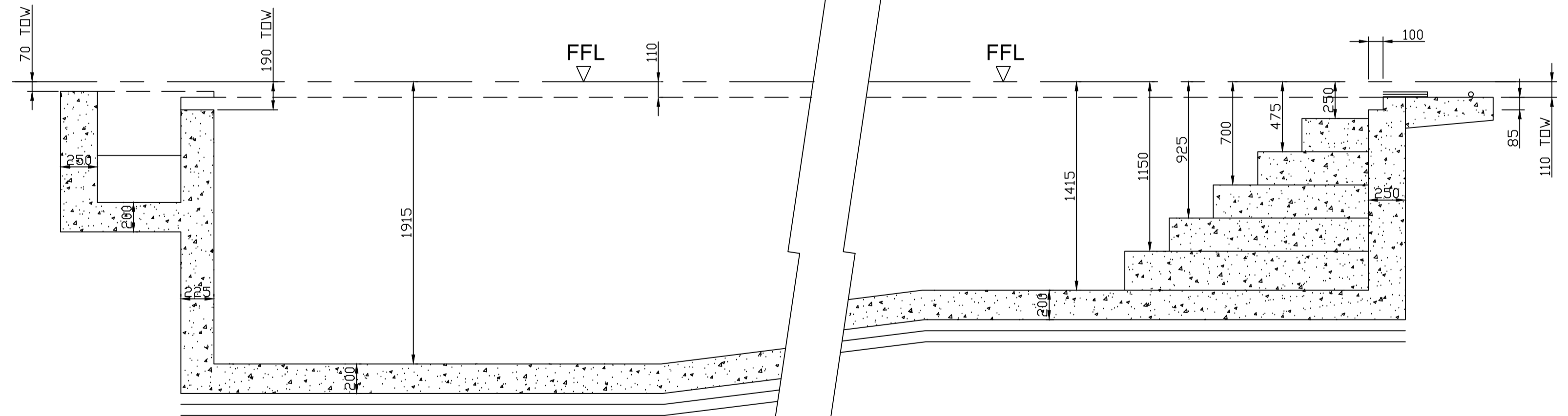
SECTION BB- POOL LENGTH
