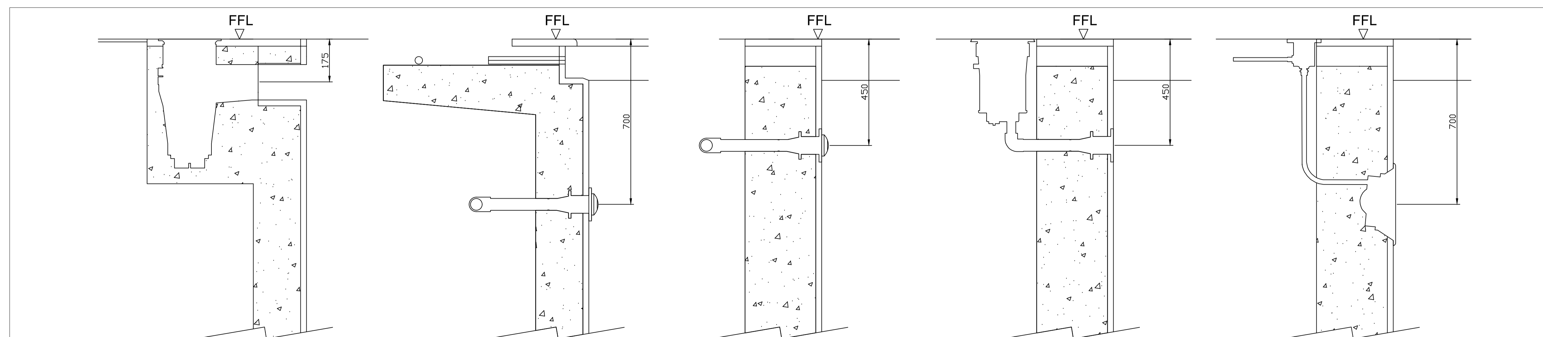
SECTIONS- POOL FITTINGS (Scale 1:10)
