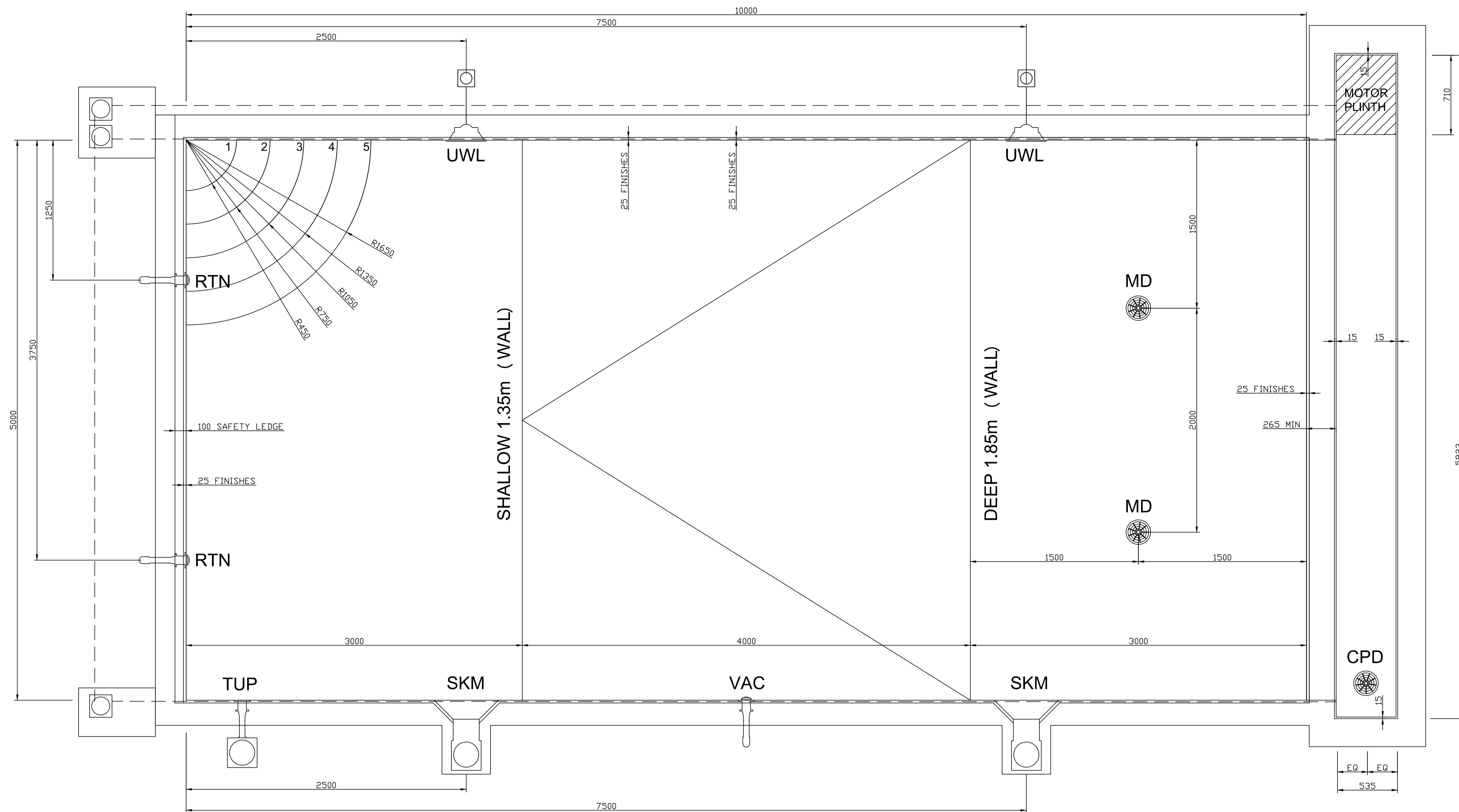
PLAN - POOL LAYOUT
