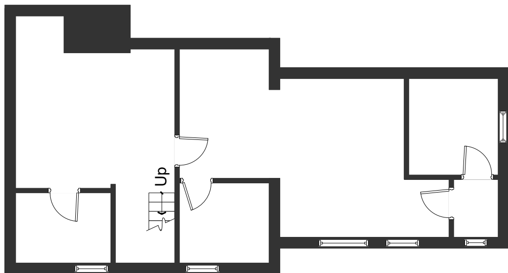
Page 1 Existing ground floor plan (1-100)
