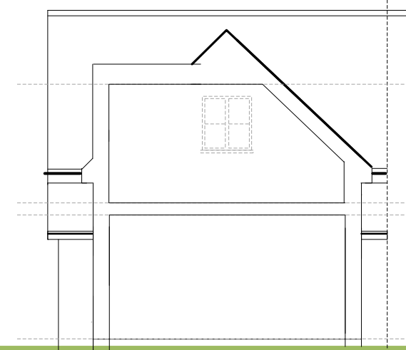
Section through dormer
