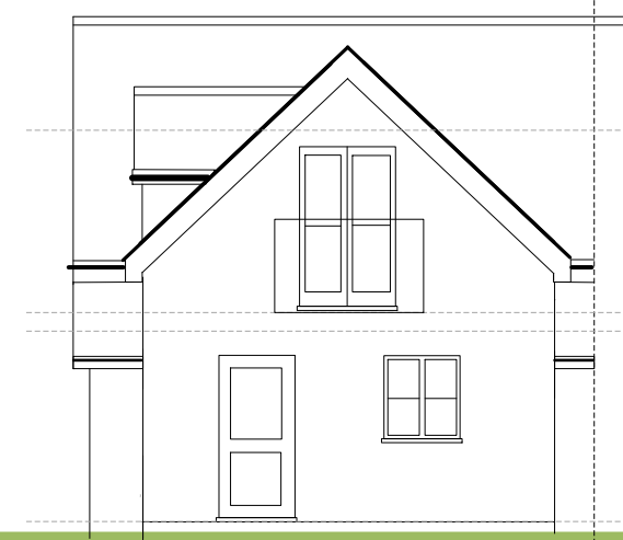
Rear elevation
