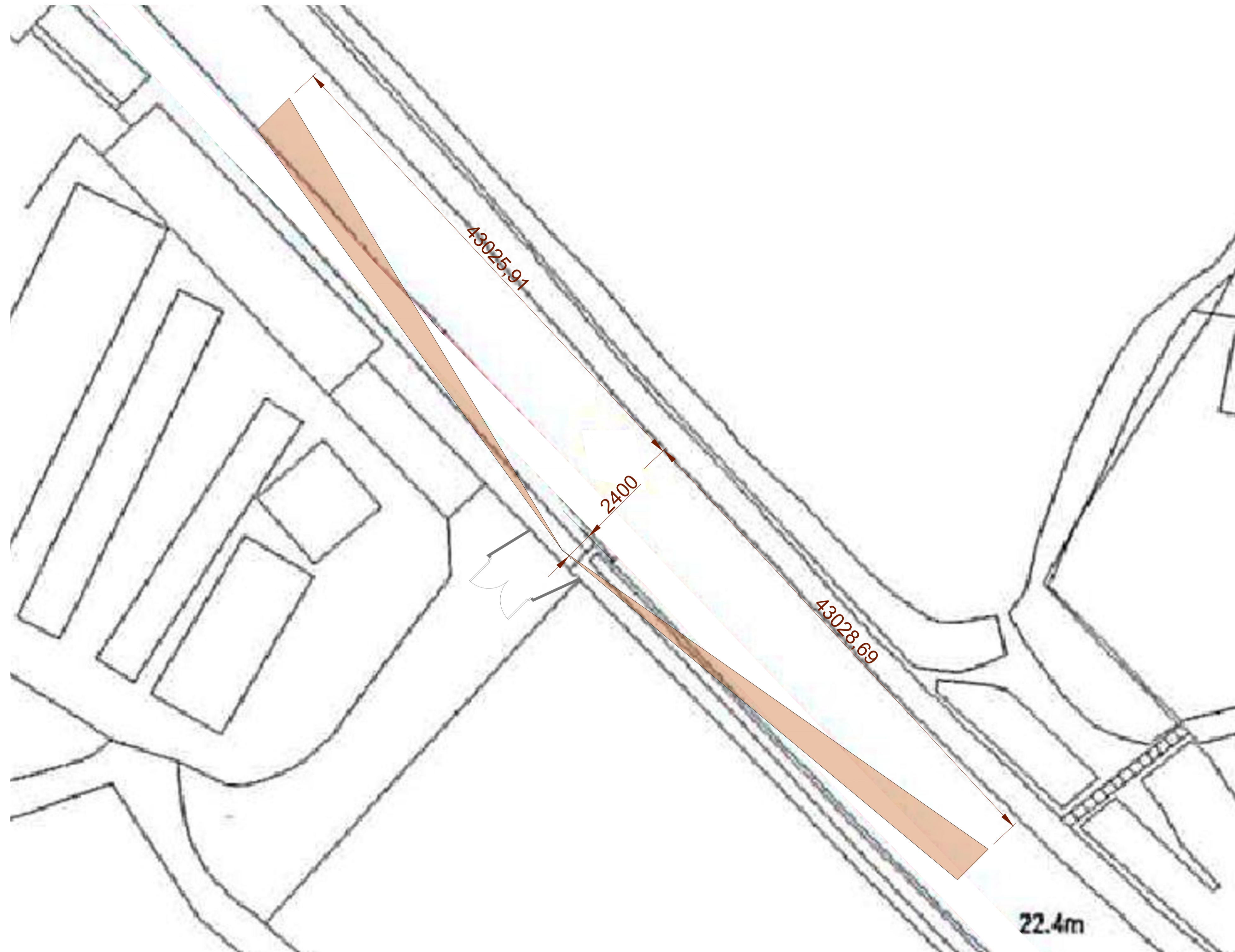
Existing Access Plan showing Vehicle Visibility Splays 1:200
