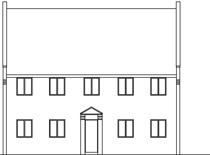
PROPOSED SOUTH ELEVATION 1-100
