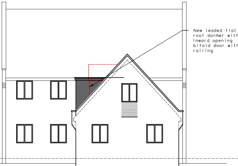
PROPOSED NORTH ELEVATION 1-100
