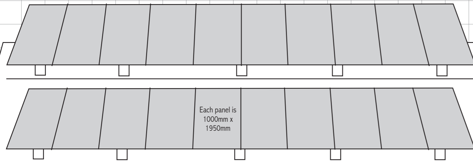
Solar panels: 2 rows of 10 panels mounted at 45 degrees on aluminium frames on an existing concrete base on the ground. South facing. Each panel measures 1000mm wide x 1950mm high.
