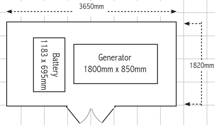
Floor plan of diesel generator block 12ft x 6ft shed housing the battery and generator
