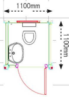
Toilet floor plan
