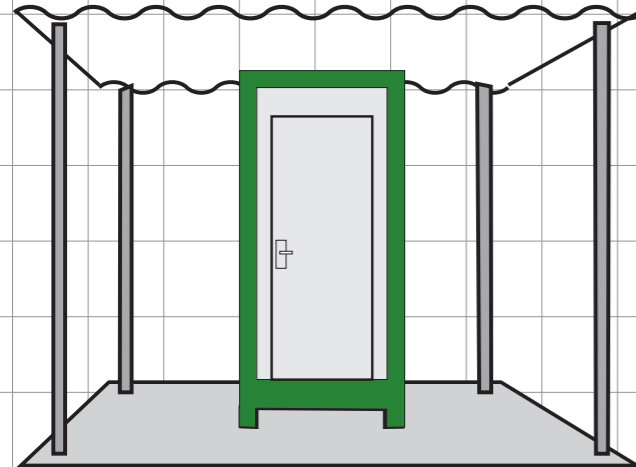
Toilet Front elevation showing roof to create an extended water catchment area. The roof will be approx 3m x 3m.
