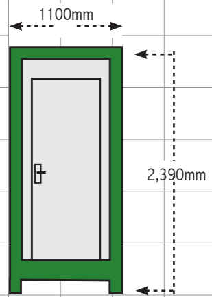
Toilet Front Elevation
