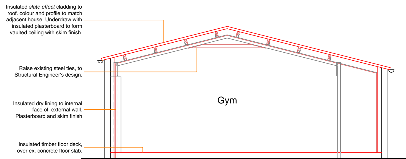
Proposed Section
