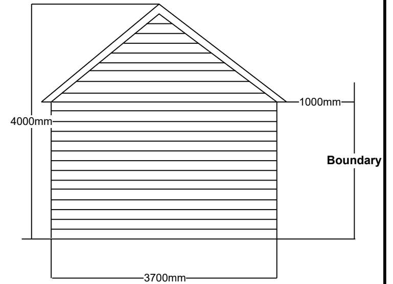
Side Elevation
