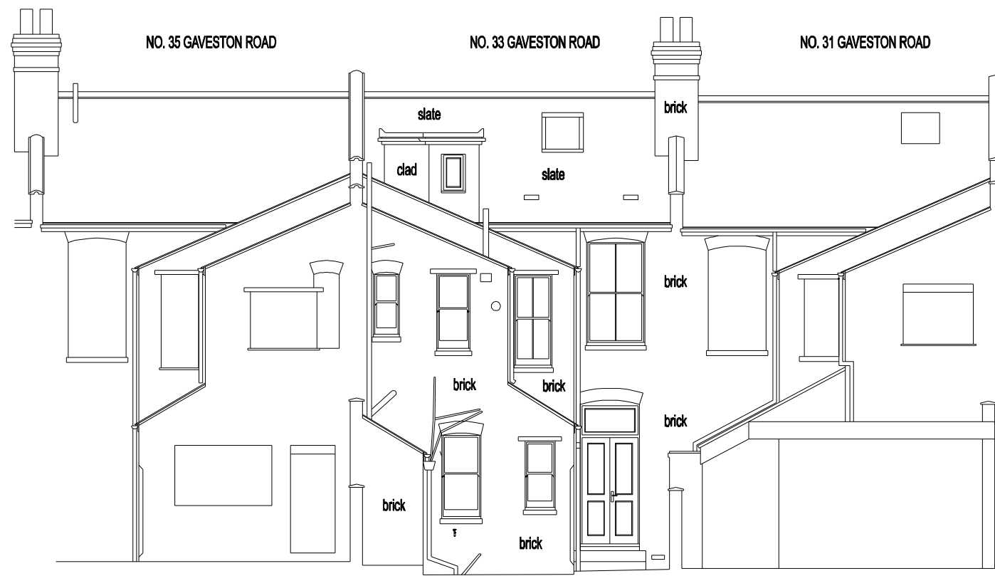
REAR ELEVATION Southwest
