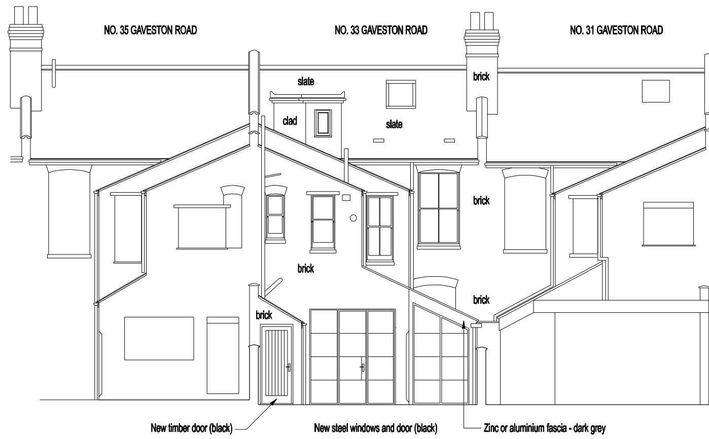
REAR ELEVATION Southwest
