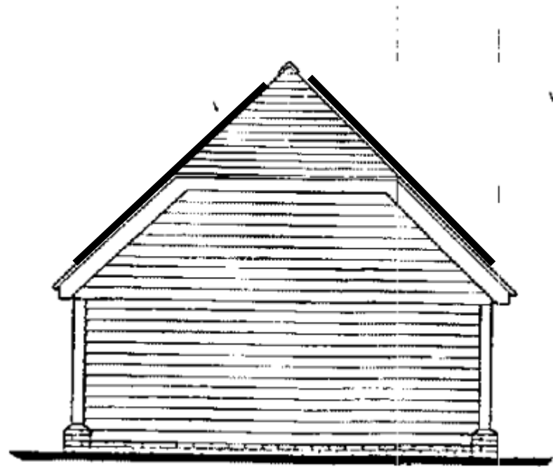
Side elevations
