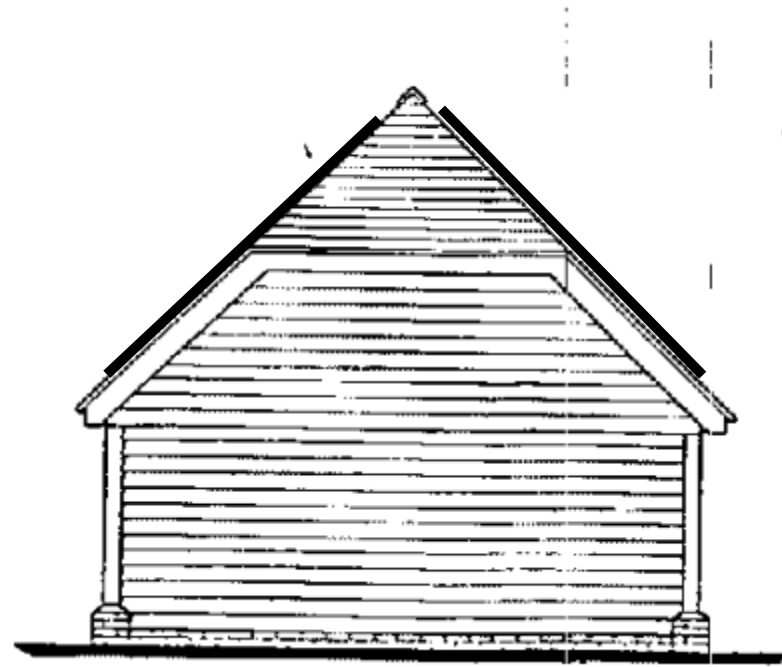
Side elevations (1:75)
