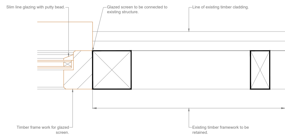
Typical Detail for Glazed Screen (1:5)
