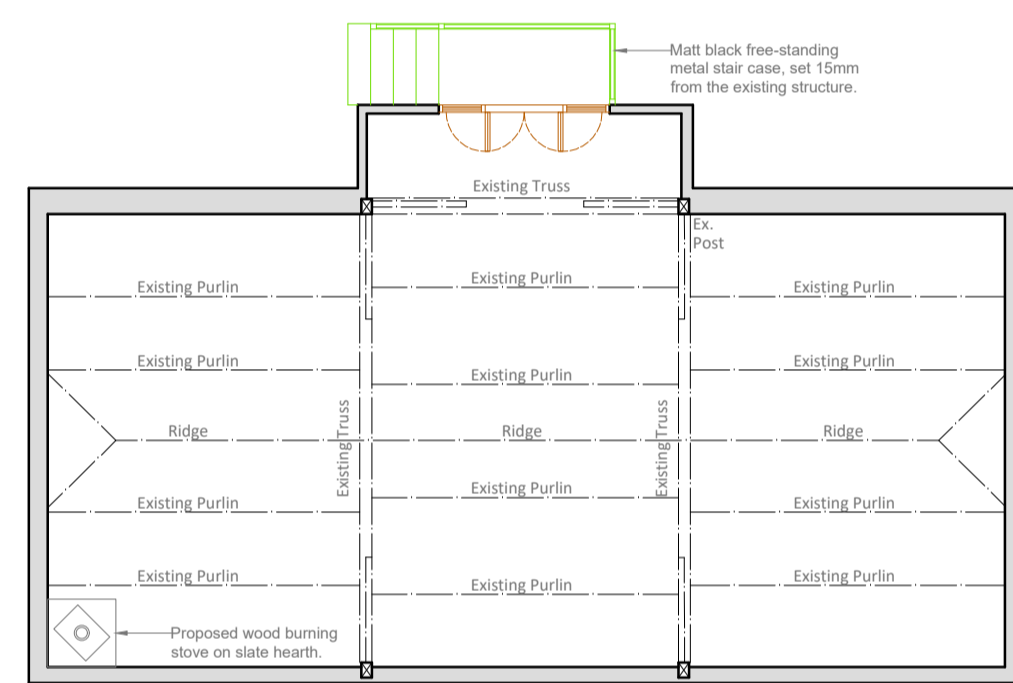
GROUND FLOOR PLAN BARN B
