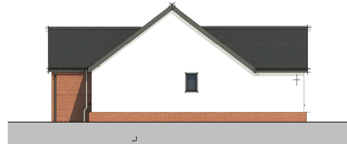
GA Left Elevation 1 : 100
