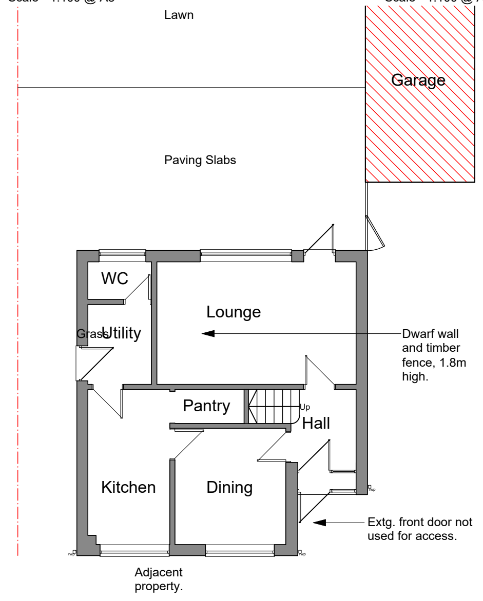
Floor Plans - Ground Floor Footprint = 56m 2 (approx.) Scale - 1:100 @ A3
