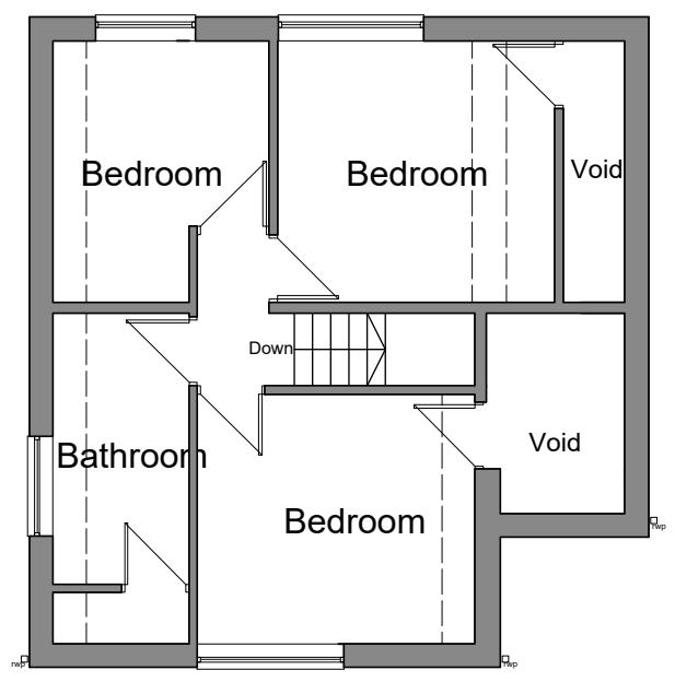
First Floor Plan Footprint = 56m 2 (approx.)
