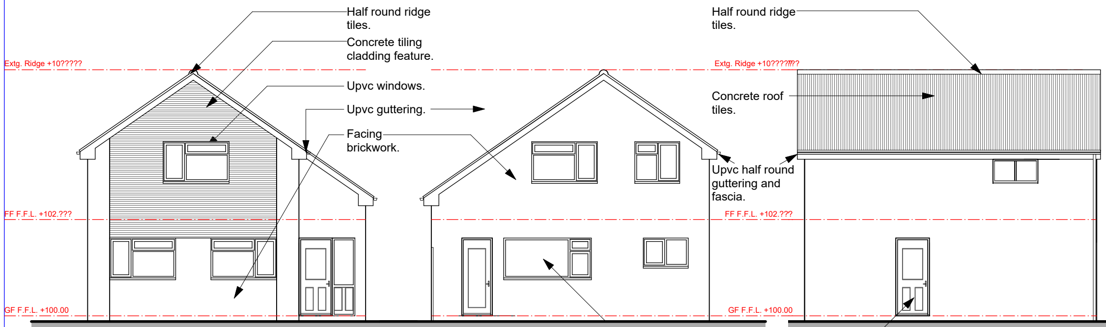
West Elevation Scale - 1:100 @ A3
