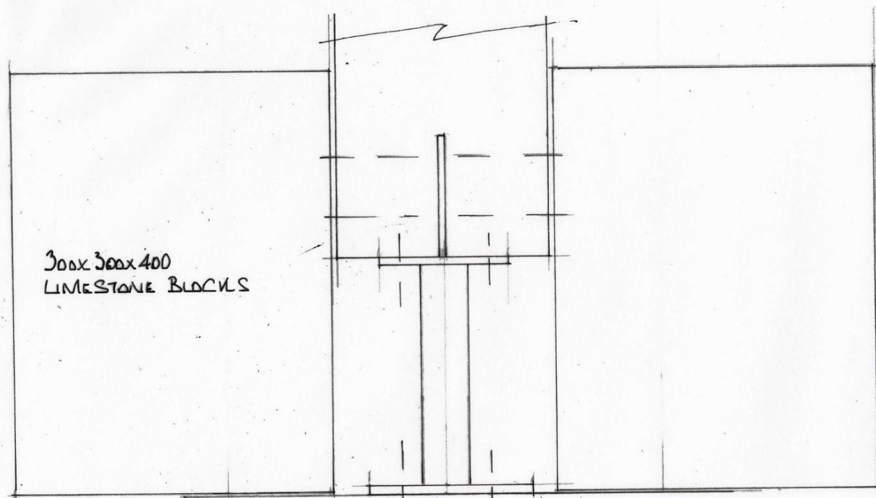
POST BASE DETAIL
