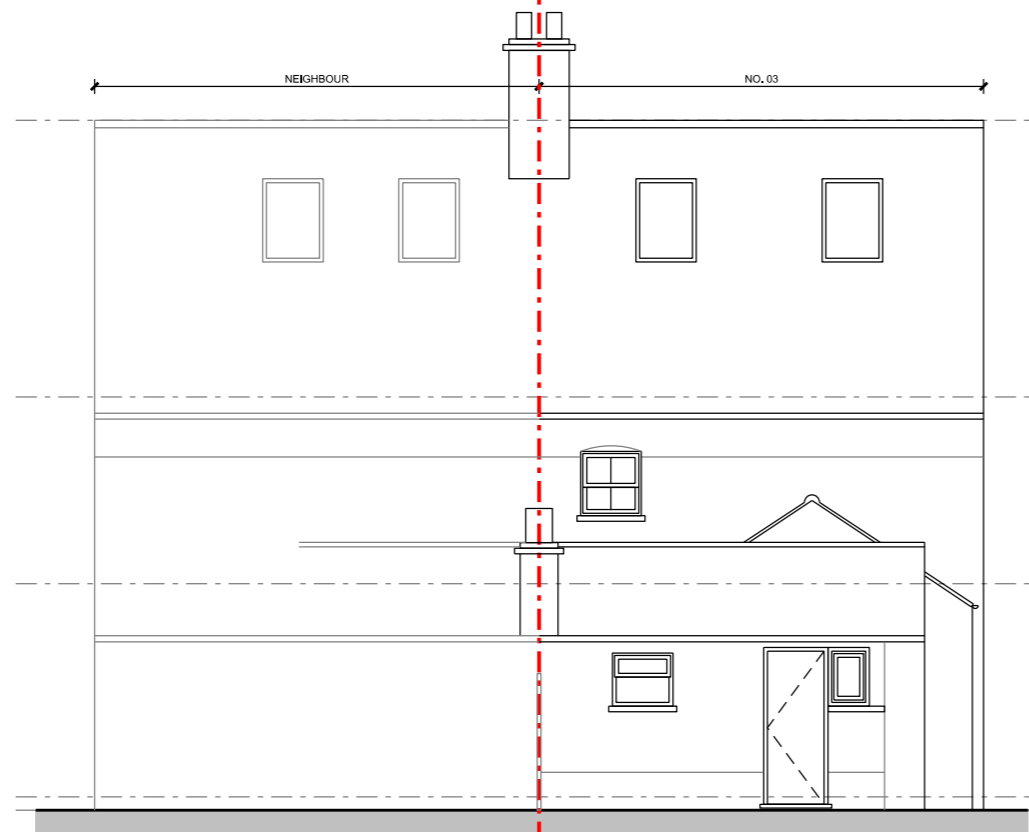
03 EXISTING WEST ELEVATION
