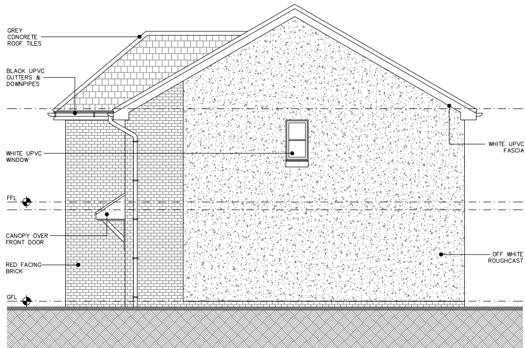
SOUTH ELEVATION
