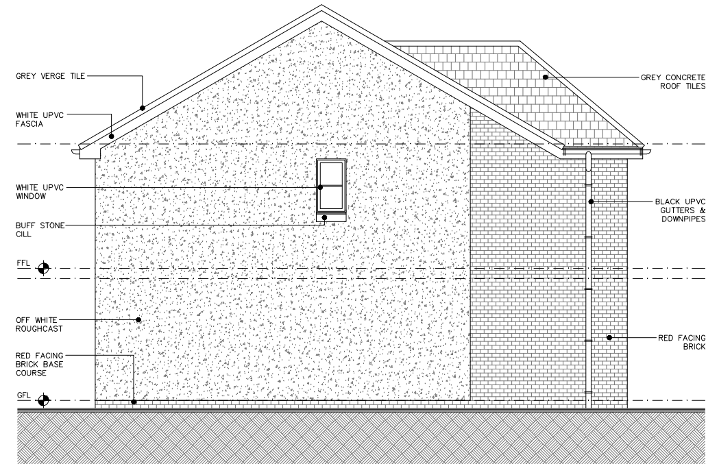
NORTH ELEVATION
