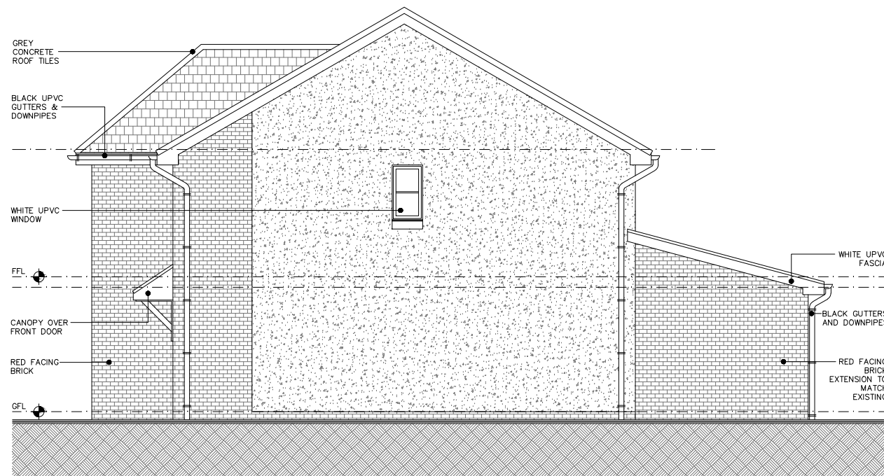
SOUTH ELEVATION
