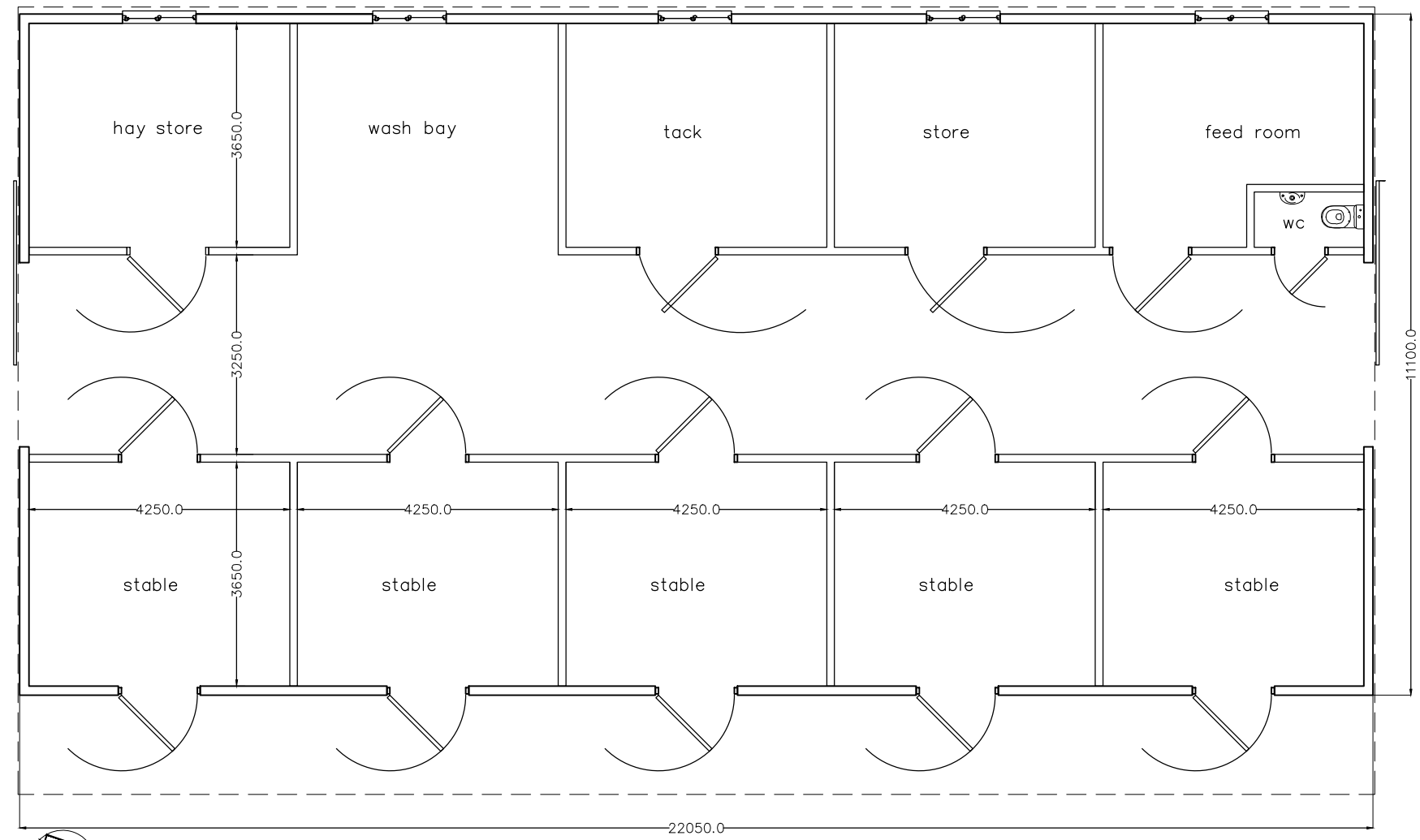
American Barn ground floor plan as proposed
