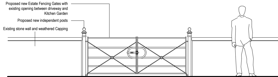
ELEVATION proposed Gates to Garden
