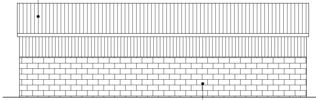
EAST ELEVATION
