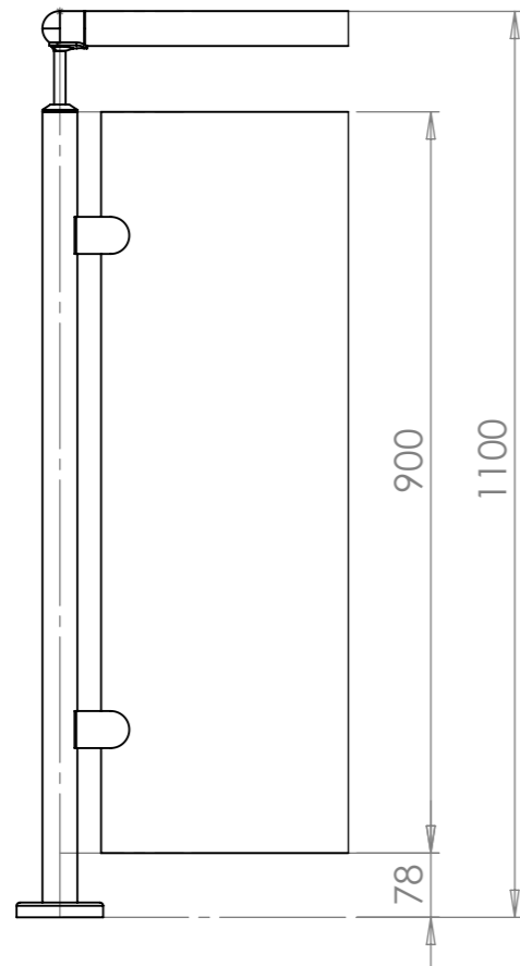
DETAIL E SCALE 1 : 10
