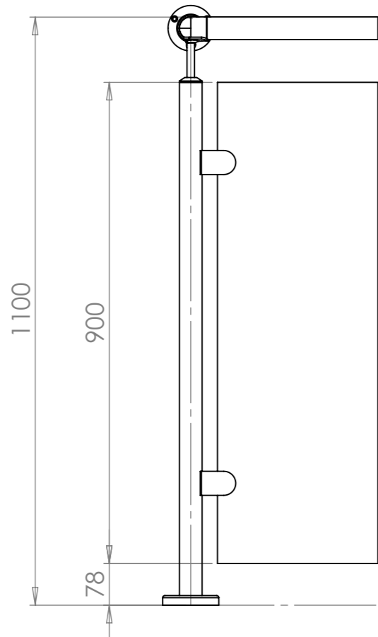
DETAIL C SCALE 1 : 10
