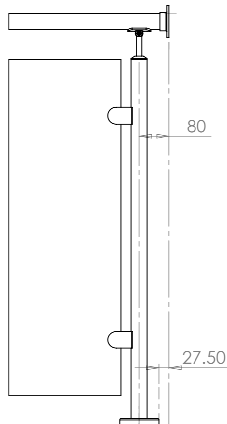
DETAIL F SCALE 1 : 10
