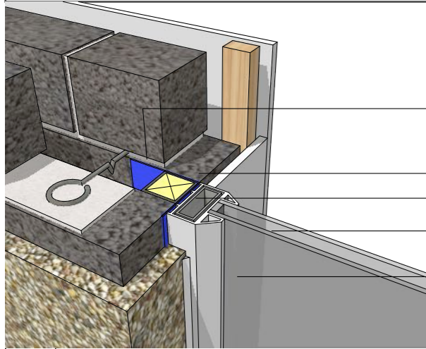
10 NEW DOOR/WINDOW REVEAL DETAIL Scale: NTS
