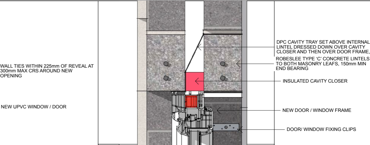
12 SECTION THROUGH WINDOW LINTEL Scale: NTS
