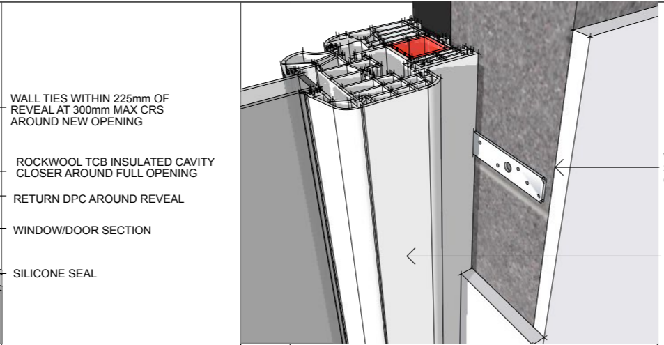
11 NEW WINDOW / DOOR REVEAL DETAIL Scale: NTS
