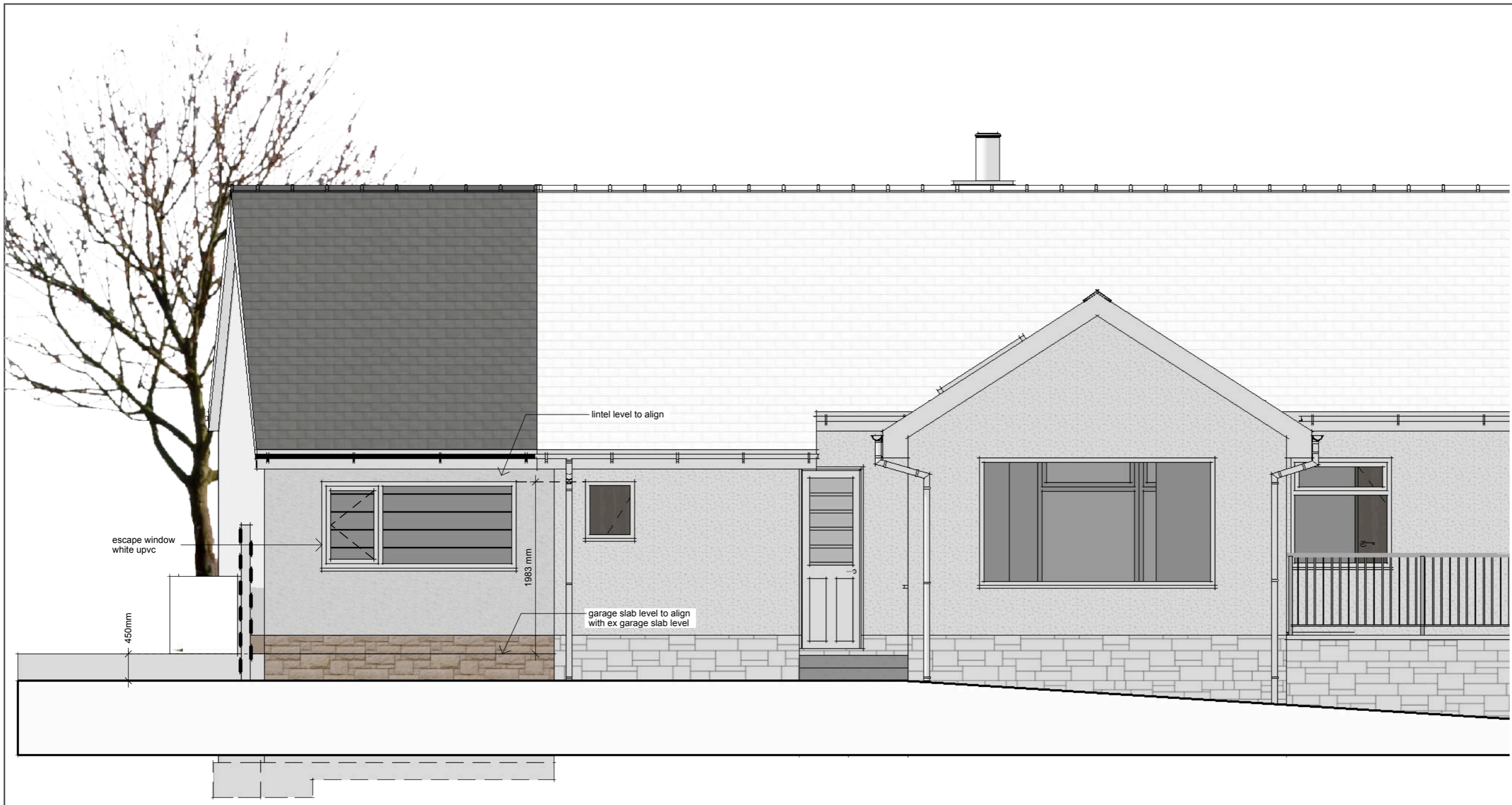
P 4 :: PROPOSED REAR ELEVATION scale: 1:50 0 1m 5m
