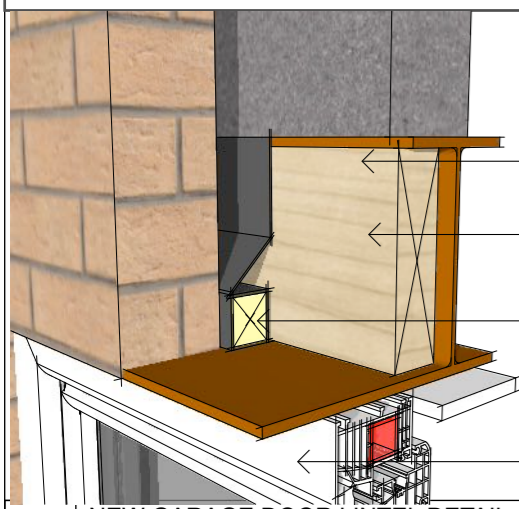
10 NEW GARAGE DOOR LINTEL DETAIL
