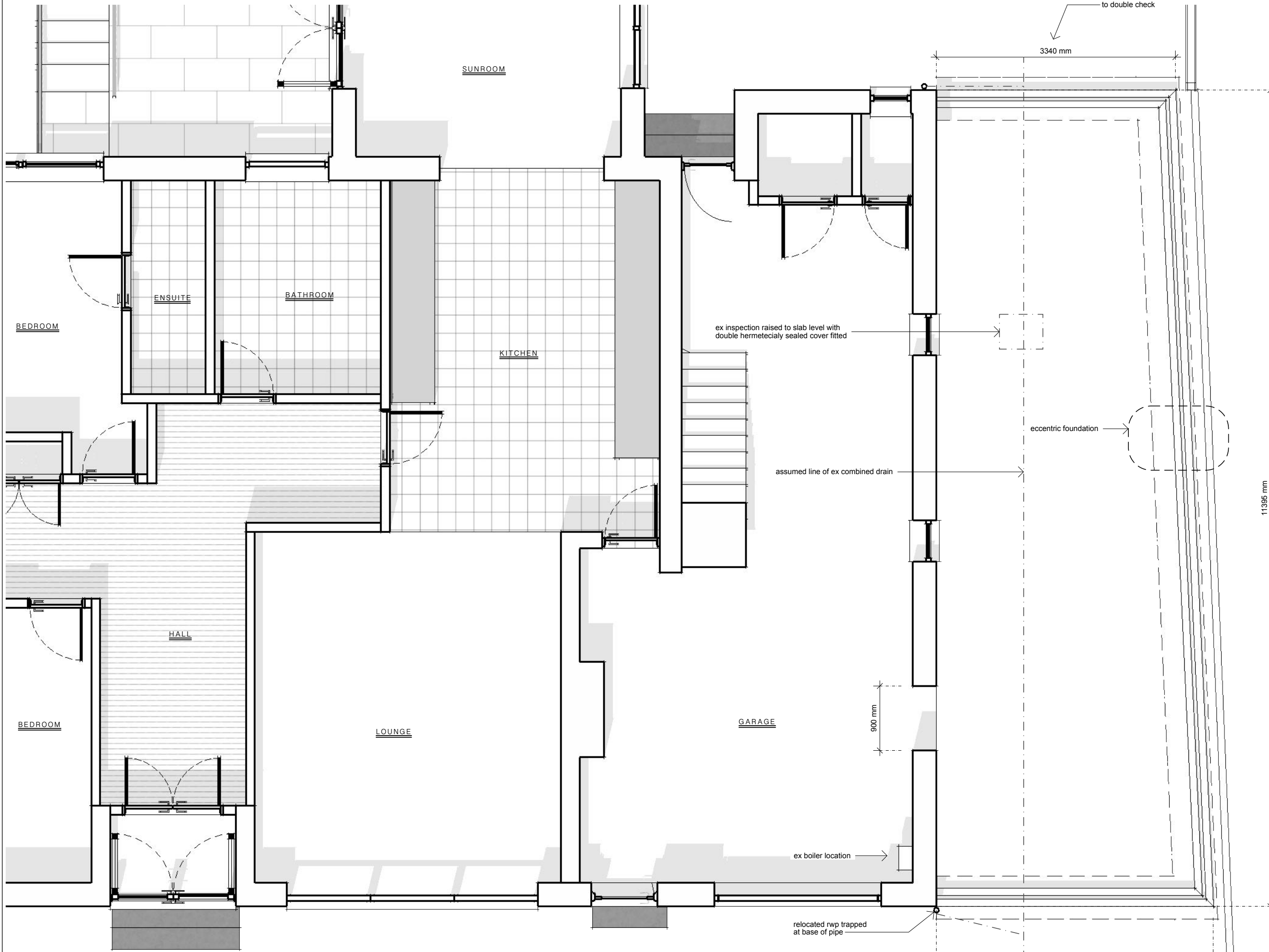
P :: PROPOSED FOUNDATION PLAN 7 scale: 1:50
