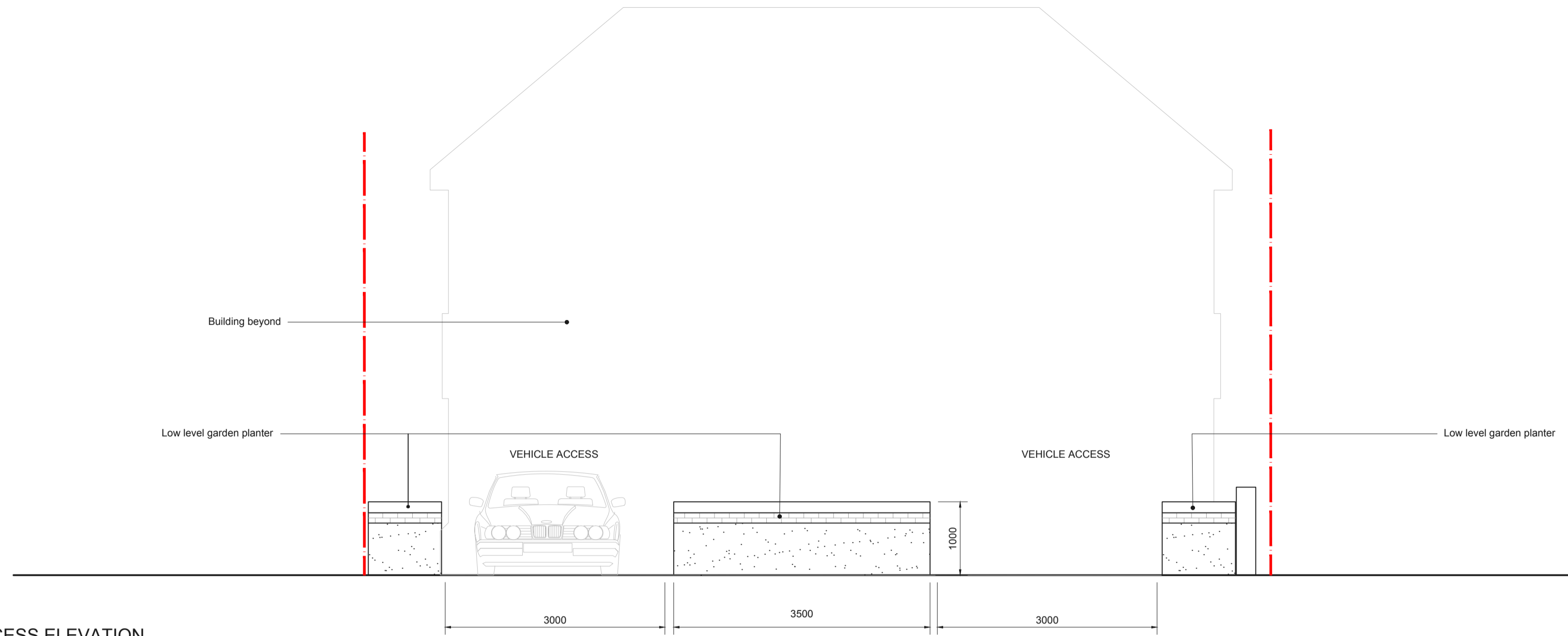
PROPOSED VEHICLE ACCESS ELEVATION 1:50
